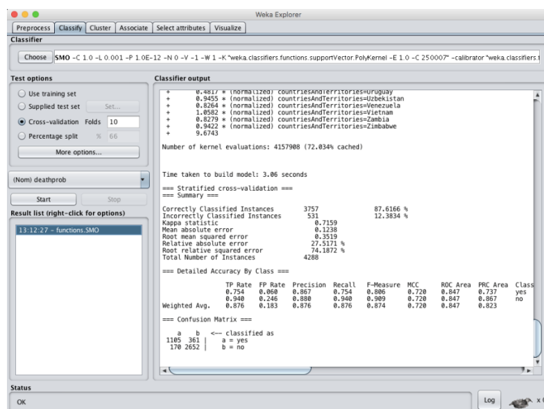
Fig.1 Processed ARFF file in WEKA.
