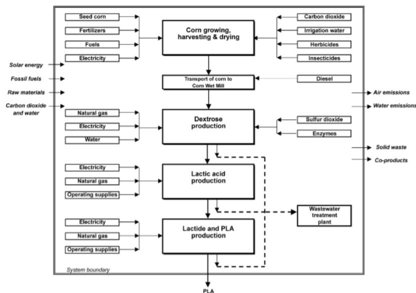
Fig. 4. Simplified flow diagram and system boundary of PLA production system [7]
