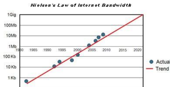
Figure 3.1. Nielsen's Law of Internet Bandwidth
