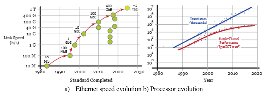
Figure 3.2. Gap between processing aptitude and link speed growth.
