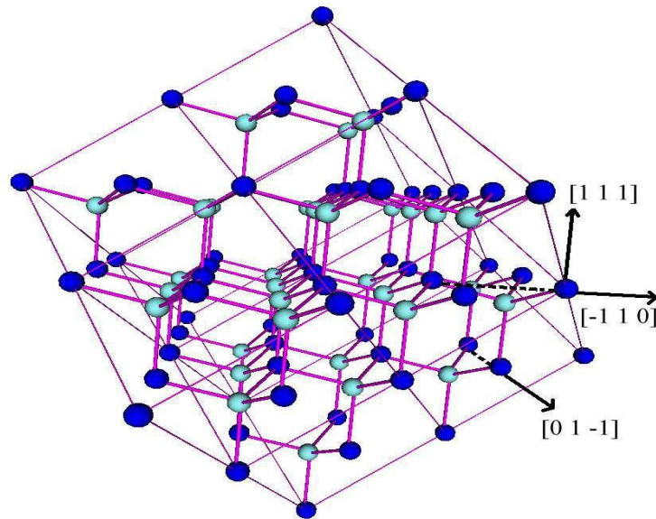
Figure 1: fcc lattice with a two-atom basis. Ga and As atoms are colored differently in the Zincblende structure and also in the diamond structure for Si, even though all atoms are identical in this case.
