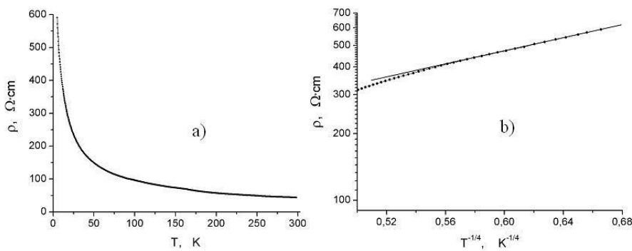
Fig.3. Temperature dependence of the resistivity in single crystals of CuGaS 2 . (a), the same in Mott coordinates (b).
